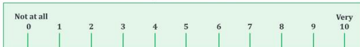
Fig 4. Readiness Ruler
